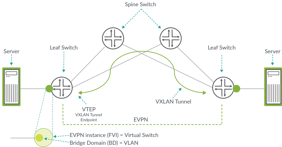
Figure 4: EVPN-VXLAN architecture
